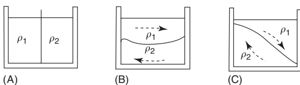
0155-F0001 Figure 1 Schematic model of fluid motion showing APE and KE concepts. The tank holds two immiscible fluids with density \rho_1 < \rho_2 . (A) Initial state; (B) state with maximum KE but minimum PE reached during the first oscillation; (C) state where KE is being converted back to PE.
