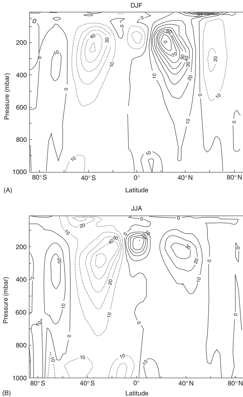
Figure 8 Zonal mean meridional flux of zonal wind [v u] for (A) December–February and (B) June–August using 1995–99 NCEP/NCAR reanalysis data. Hadley cell fluxes are apparent in the tropics, while eddy fluxes predominate in midlatitudes.
