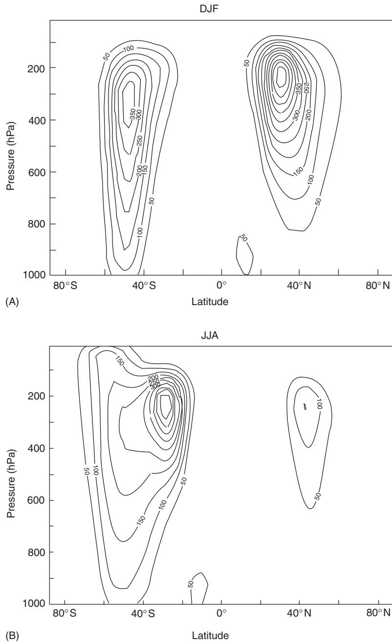
0155-F0004 Figure 4 Zonal mean kinetic energy density for (A) December–February and (B) June–August using 1979–99 NCEP/NCAR reanalysis data. The contour interval is 50 \text{ kg s}^{-2} \text{ m}^{-1} .
