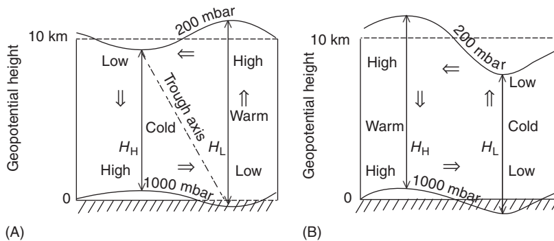
Figure 6 Highly idealized schematic illustration of a midlatitude frontal cyclone during (A) baroclinic growth and (B) baroclinic decay. The 1000 and 200 mbar surfaces are marked. Areas of relatively warmer and colder air at an isobaric level are noted. Double-shafted arrows indicate the relevant part of the ageostrophic circulation. The dot-dashed line in (A) shows the trough axis through the troposphere.
