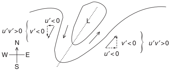
0155-F0009 Figure 9 Schematic illustration of how a horizontal tilt of the trough axis (dotted line) leads to a net meridional transport of eddy zonal momentum. Primes denote winds with the zonal average removed. In this case the zonal average eddy momentum flux is northward. In contrast, a low that is symmetric about a north–south axis has u'v' contributions on the east and west sides that cancel in the zonal mean.
