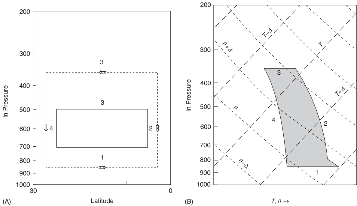
0155-F0002 Figure 2 Interpretation of the Hadley circulation as a Carnot cycle. (A) Meridional cross-section showing the idealized circulation. The dashed line shows an average path followed by the parcels with numeric labels for each leg. (B) Skew T - \ln P plot of the thermodynamic changes along each of the four legs drawn in part (A). The shaded area is proportional to the energy converted from PE to KE.
