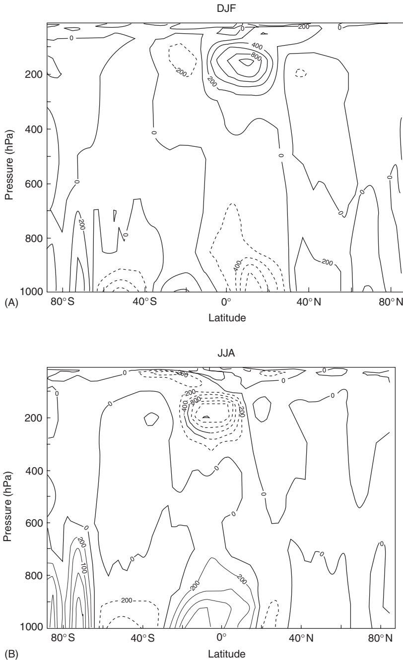
0155-F0007 Figure 7 Zonal mean meridional flux of potential temperature [v\theta] for (A) December–February and (B) June–August using 1995–99 NCEP/NCAR reanalysis data. Hadley cell fluxes are apparent in the tropics, while eddy fluxes predominate in midlatitudes.
