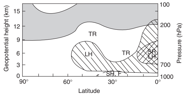
Figure 5 Schematic distribution of the primary sources of diabatic heating. Solar radiation (SR) heating rate is greatest near the equatorial lower troposphere. Cross-hatching indicates SR > 1 K d^{-1} . The area with terrestrial radiation (TR) cooling rate magnitude < 1 K d^{-1} is shaded. Terrestrial radiation labels are placed where relative extremes of cooling occur. Latent heat is released in the lower and middle troposphere in regions where rainfall is relatively heavier, with relative maxima indicated by the latent heat label (LH). The area with LH exceeding 1 K d^{-1} is marked with hatching bounded by a chain curve. Surface sensible heat flux exceeds 1 K d^{-1} (dashed line) in the subtropics.
