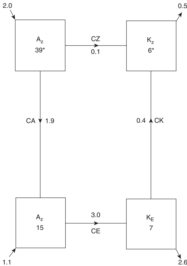
Figure 11 Energy “box” diagram showing reservoirs of zonal mean APE ( A_z ) and KE ( K_z ); eddy APE ( A_e ) and KE ( K_e ); net energy conversions (CA, CE, CK, CZ); and net diabatic generation or destruction. Global and annual average values indicated. The reservoirs are in units of 10^5 J m^{-2} and the conversions and diabatic processes have units of W m^{-2} . The conversions are given letter labels for future reference. The numbers are highly idealized and drawn from several sources with adjustments made to round off and balance input and output. The two numbers with asterisks are estimates made by the author using 1979–99 NCEP/NCAR reanalysis data.
