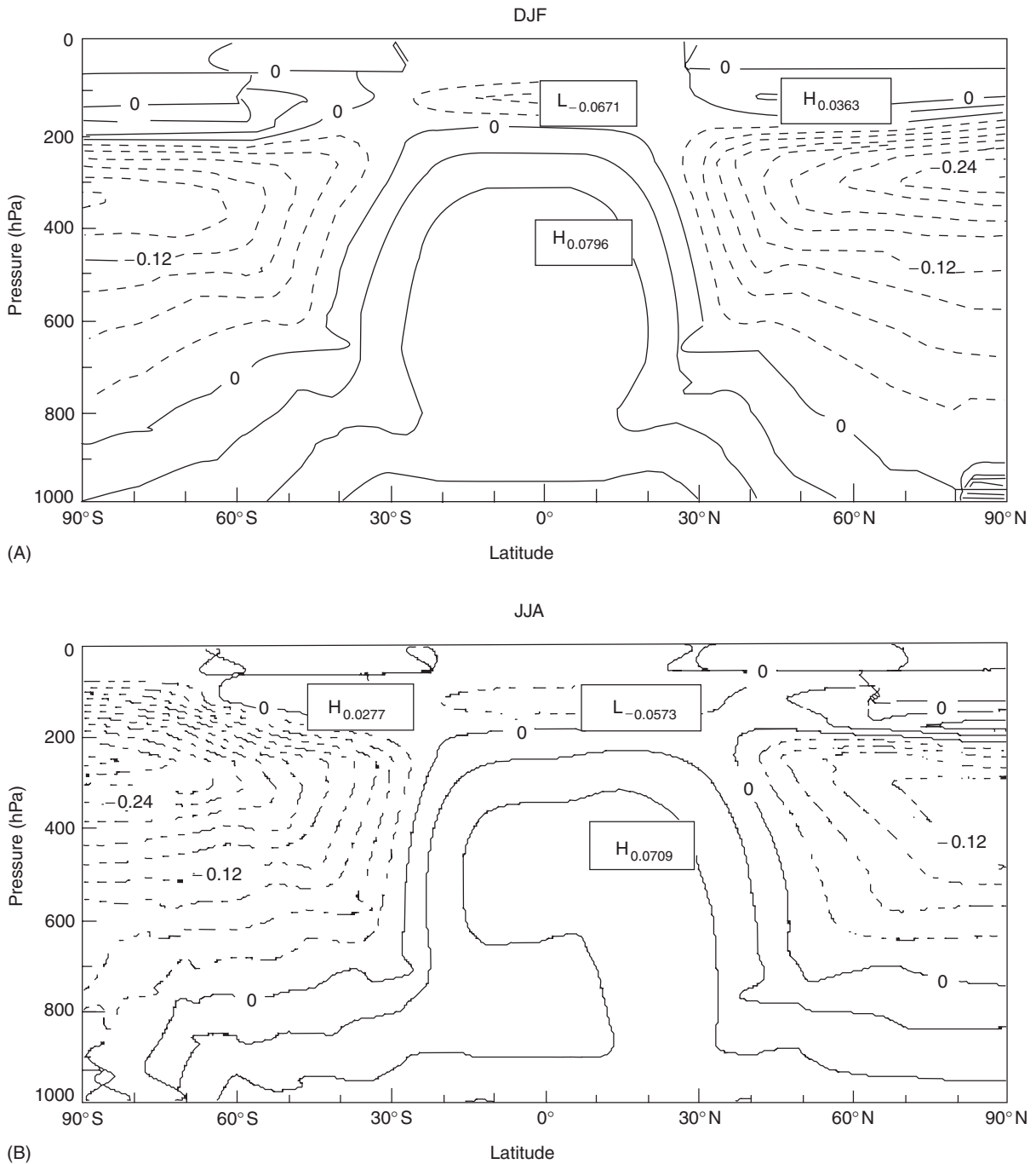
0155-F0003 Figure 3 Zonal mean efficiency factor [\varepsilon] for (A) December–February and (B) June–August. [\varepsilon] is estimated from zonal mean 1979–99 National Center for Environmental Prediction/National Center for Atmospheric Research (NCEP/NCAR) reanalysis data. The contour interval is 0.03.
