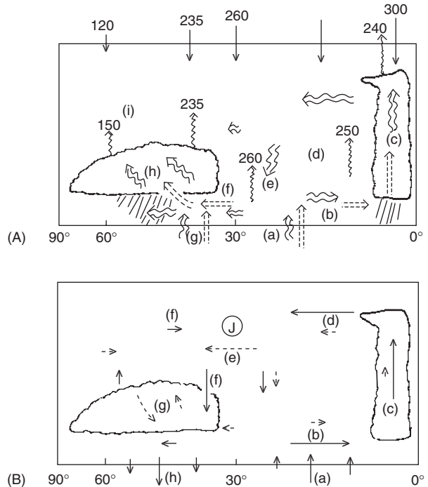
Figure 12 (A) Schematic meridional cross-sections of the atmospheric cycle of APE and heat. Arrow lengths are intended to suggest relative magnitudes. Single-shafted arrows depict radiation (straight for absorbed solar; wavy for terrestrial emitted to space) with representative numerical values given in W m^{-2} . Double-shafted arrows depict heat fluxes (dashed for latent; wavy for sensible heat). Letters correspond to distinct parts of the cycle. Solar radiation (a) is absorbed in the tropics and subtropics, then that heat energy is transported (b) equatorward. Latent heat (c) is converted to sensible heat in the ICZ then transported poleward (d) in the upper troposphere. Sinking in the Hadley cell (e) brings heat downward. Eddy fluxes (f) extract heat from the subtropics and are augmented by surface fluxes (g) at WBCs. Heat is mixed upward vertically (h) in frontal cyclones, whereupon a net loss occurs to space (i). (B) Similar to (A) except for the KE and momentum cycle. Arrow lengths are intended to suggest relative magnitude of momentum transport. Momentum transport in the troposphere is separated into mean meridional cells (solid arrows) and eddies (dashed arrows). Letters correspond to these parts of the cycle: Slowing down surface easterlies impart westerly momentum (a) into the tropical boundary layer. That momentum is transported equatorward (b) then upward (c) in the ICZ convection. The upper Hadley cell transports the momentum (d) poleward. Eddies further transport the momentum (e) poleward, out of the subtropics, while the Ferrel cell (f) both opposes the eddy flux and mixes some momentum downward. Frontal cyclones also have a net downward mixing (g) of westerly momentum that is lost by friction at the surface (h). The transport creates westerly momentum convergence in the subtropics and midlatitudes forming a subtropical jet (J) and a KE maximum there.
