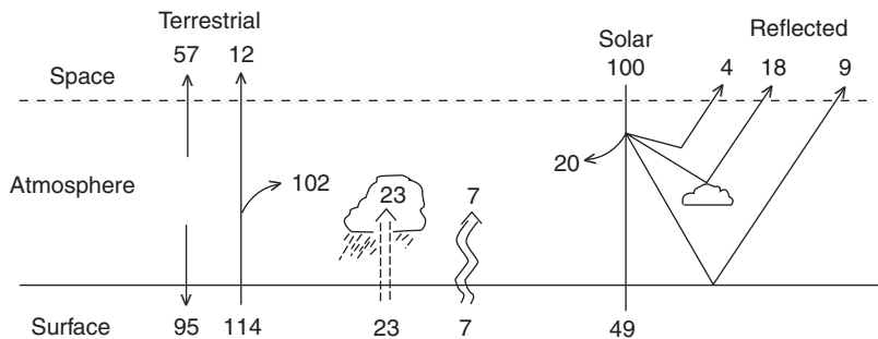
0155-F0010 Figure 10 Global average energy balance expressed as percentages of the solar radiation striking the top of the atmosphere. Estimates of the solar constant vary, but the 100 units in the figure correspond to \sim 342 \text{ W m}^{-2} . Right side: solar radiation processes showing amounts reflected and absorbed. Middle: surface sensible heat flux (wavy arrow) and surface latent heat flux (dashed arrow). Left side: terrestrial radiation processes showing emission, transmission, and absorption. (Data in the figure come from several sources, but primarily from Kiehl J and Trenberth K, (1997) Bulletin of the American Meteorological Society 78: 197–208.)
