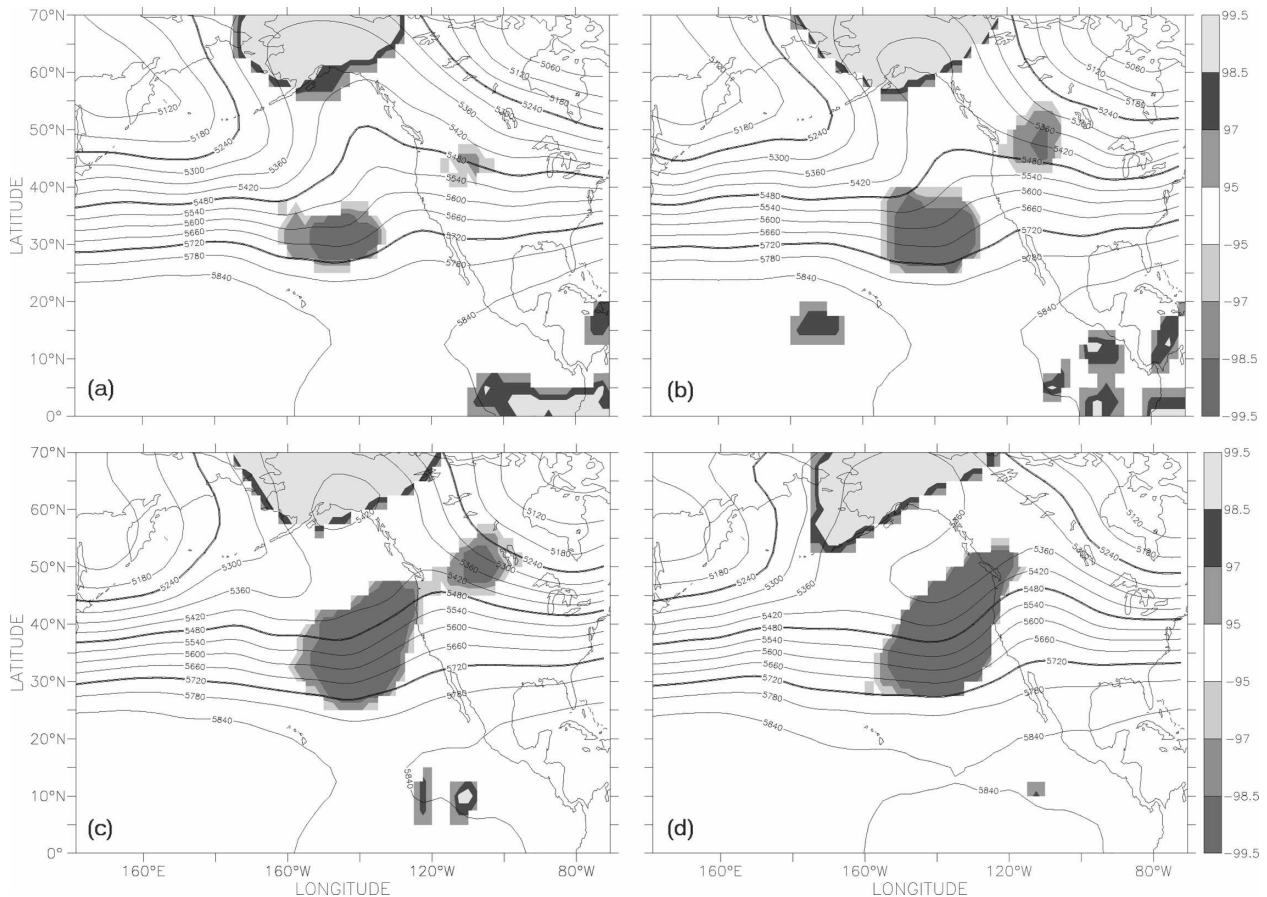
FIG. 5. Similar to Fig. 2 but showing 500-hPa geopotential height pattern typical of the heaviest prolonged rain target group. Contours use 60-m intervals for the target group ensemble mean. Composite maps shown are (a) 72, (b) 48, and (c) 24 h prior to the onset of the heavy rain, and (d) at the time of event onset.
