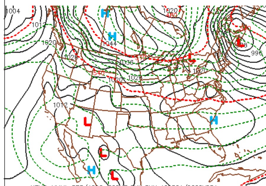
NEMS-NMMb PRS/1000-500MB THK SUN 150201/0000V054 INITIAL TIME = 150129/1800F054
