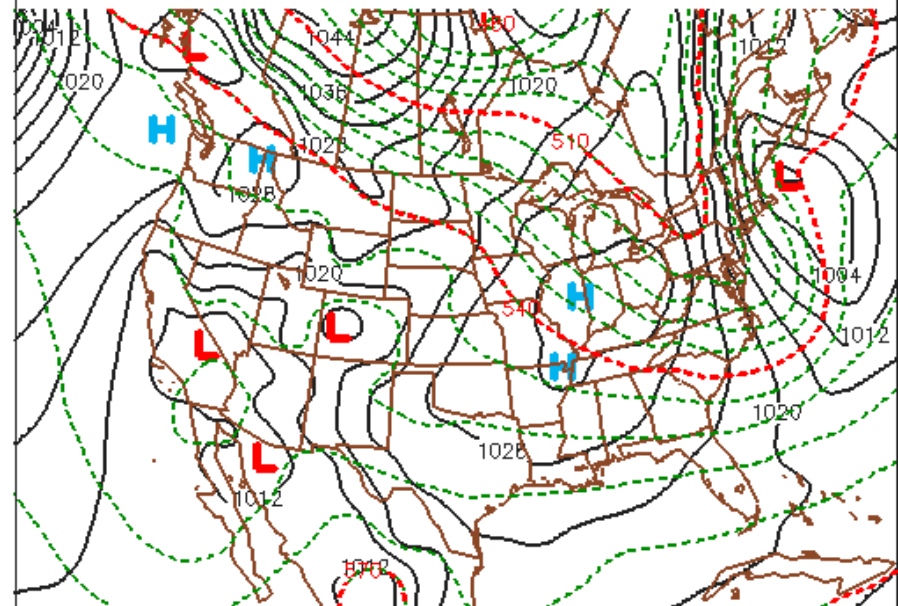
NEMS-NMMb PRS/1000-500MB THK SAT 150131/0000V030 INITIAL TIME = 150129/1800F030
