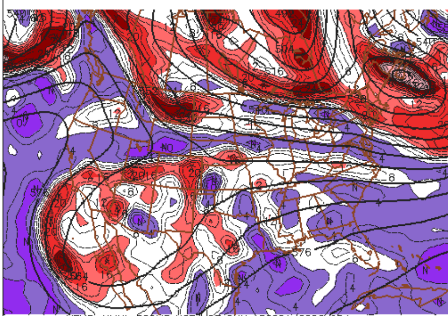
NEMS-NMMb 500MB HGT/VOR SUN 150201/0000V054 INITIAL TIME = 150129/1800F054
