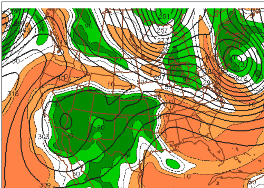
NEMS-NMm6 700MB HGT/RH SAT 150131/1200V042 INITIAL TIME = 150129/1800F042
