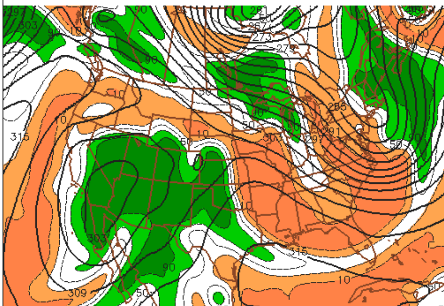
NEMS-NMMb 700MB HGT/RH SAT 150131/0000V030 INITIAL TIME = 150129/1800F030
