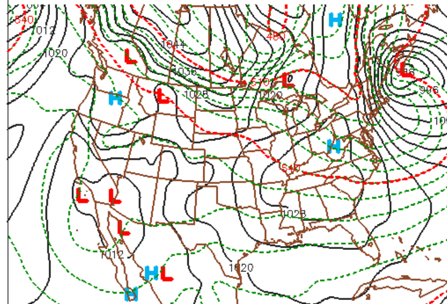
NEMS-NMm6 PRS/1000-500MB THK SAT 150131/1200V042 INITIAL TIME = 150129/1800F042
