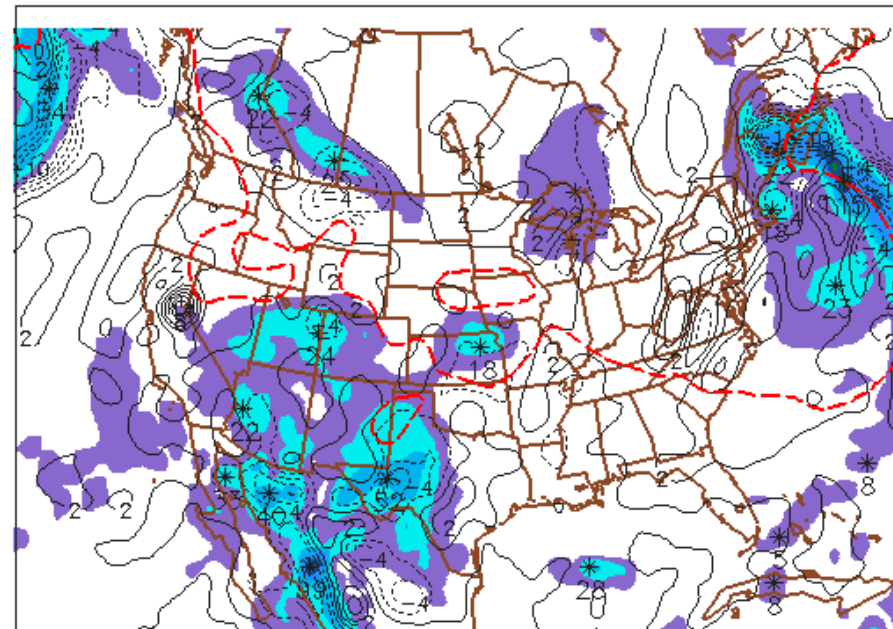
NEMS-NMm6 6HR PRECIP ENDING SAT 150131/1200V042 NEMS-NMm6 700MB OMEGA/850MB OC SAT 150131/1200V042
