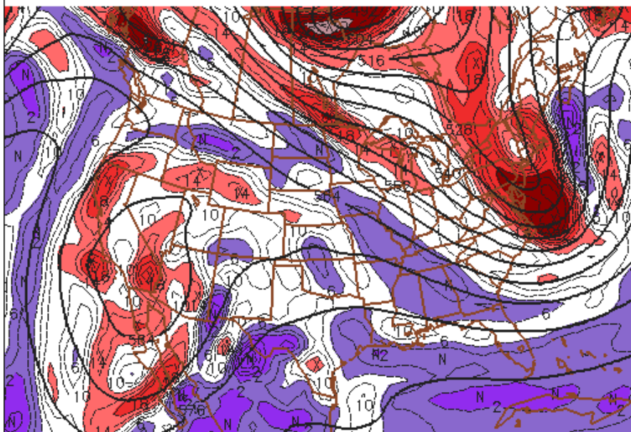
NEMS-NMMb 500MB HGT/VOR SAT 150131/0000V030 INITIAL TIME = 150129/1800F030
