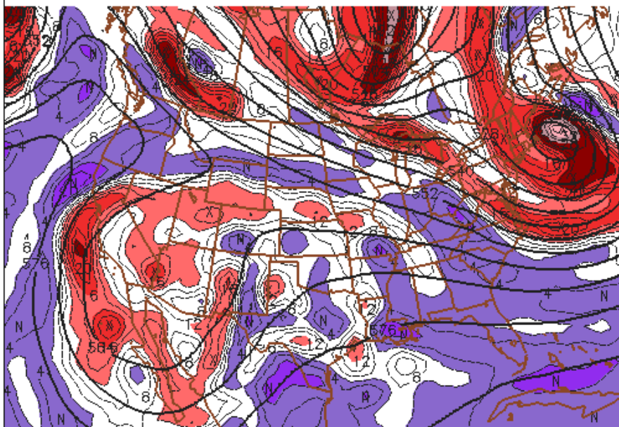
NEMS-NMm6 500MB HGT/VOR SAT 150131/1200V042 INITIAL TIME = 150129/1800F042
